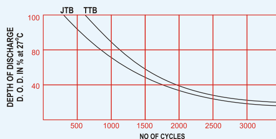
TYPICAL DISCHARGE CHARACTERISTICS CURVES OF D-FORCE TUBULAR BATTERIES AT VARIOUS DEPTH OF DISCHARGE (D. O. D.)
